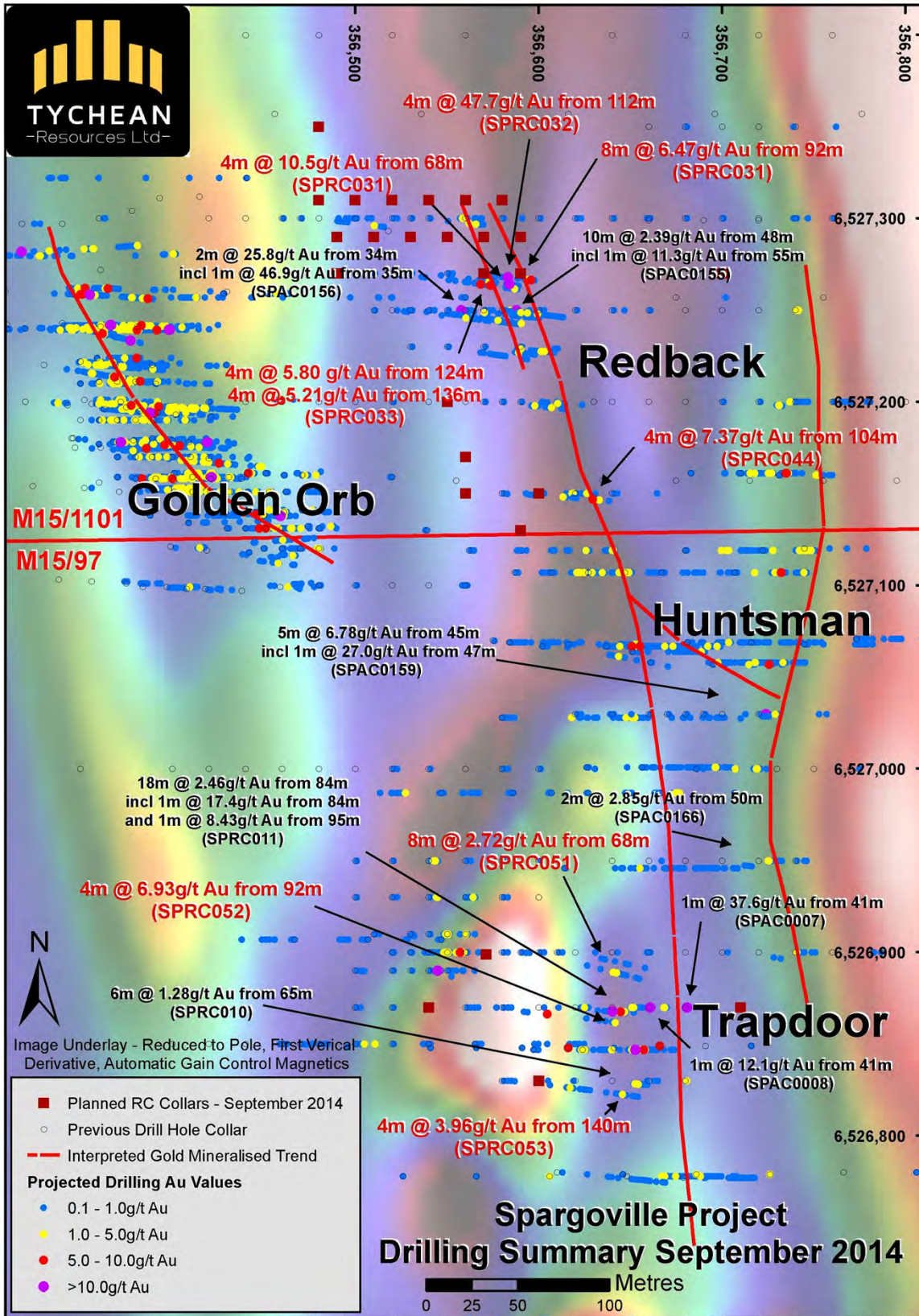
Figure 2 – Spargoville Gold Project – Redback-Trapdoor Drilling Summary Plan
